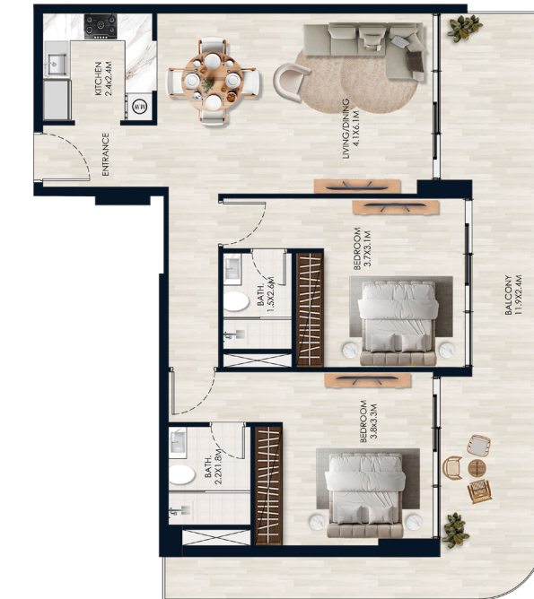
Floor Plan
